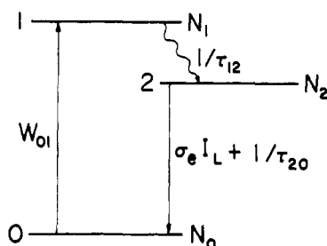
Figure 2. Three-level laser medium N_i is the population density of level i , \tau_{ij} are lifetimes, W_{01} is the pumping rate, \sigma_e is the stimulated emission cross section, and I_L is the laser intensity.
