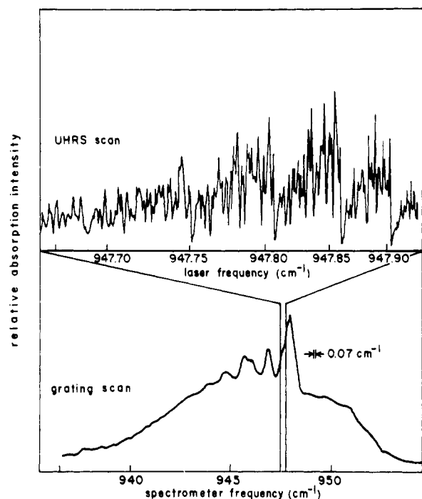
Figure 5. Spectrum of the \nu_3 band of \text{SF}_6 , obtained with a conventional high-resolution spectrometer and with a tunable PbSnTe diode laser (after Hinkley 49 ).
