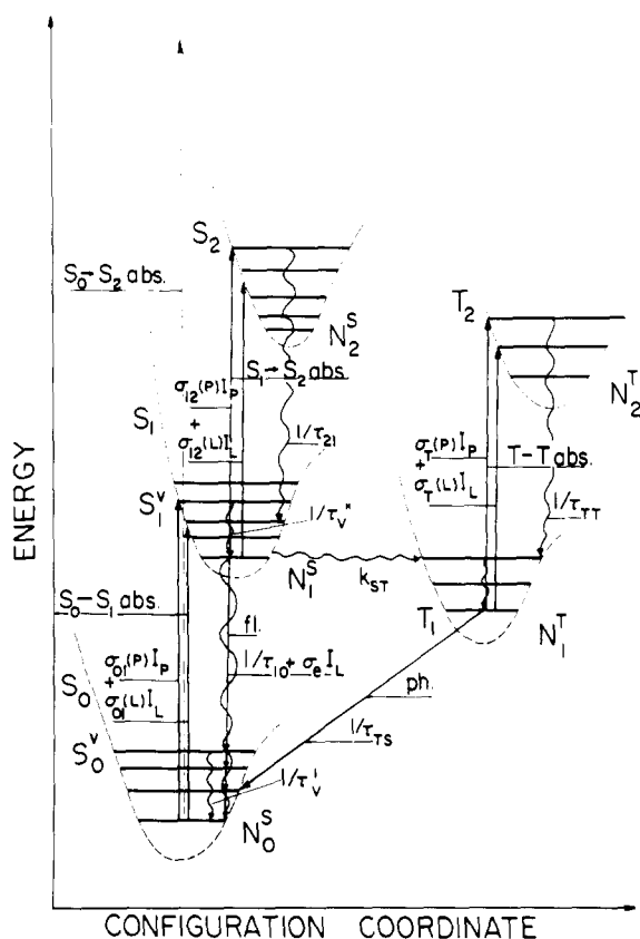
Figure 8. Diagram of photophysical and kinetic processes occurring in a solution of large organic molecules, typical examples being dye compounds. S_i and T_i designate, respectively, singlet and triplet states having populations N_i^S and N_i^T . In the singlet manifold the absorption (abs) rates are \sigma_{ij}(p)I_p and \sigma_{ij}(L)I_L at the pumping (p) and, if applicable, at the dye laser (L) frequency; in the triplet manifold the absorption rate is designated by \sigma_T I . The lifetime of the vibrational level v in the ground electronic state is \tau_v , and \tau_v' in the excited state; \tau_{10} is the fluorescence (fl) and \tau_{TS} the phosphorescence (ph) lifetime; \tau_{21} and \tau_{TT} denote nonradiative lifetimes and k_{ST} is the intersystem crossing rate constant.
